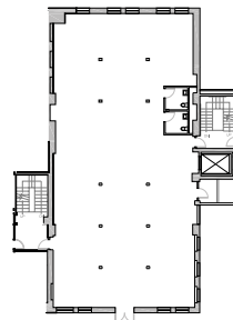
BASE FLOORPLAN
